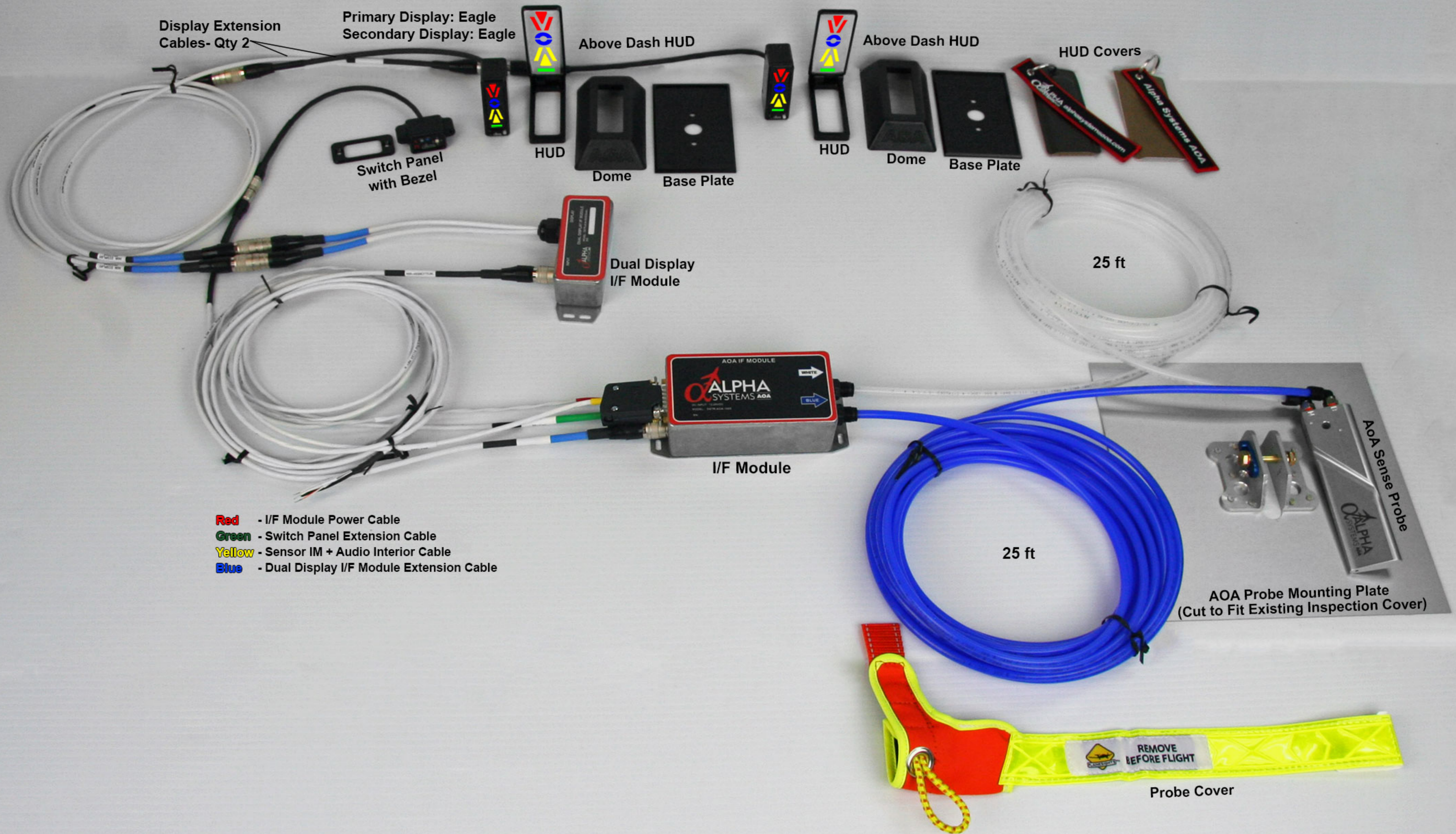
Alpha Systems AOA Eagle Dual Above Dash HUD System Diagram DSTR-AOA-9600KDUAL-(ADH)
