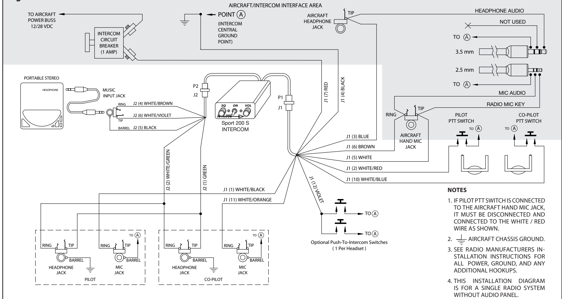
Sport 200S – ICOM A3, A6, A22, A24 Radio Installation Wiring Diagram
