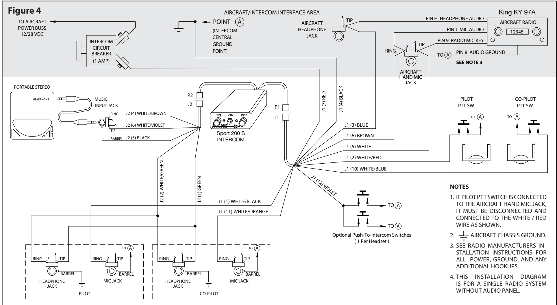
Sport 200S – King KY 97A Radio Installation Wiring Diagram
