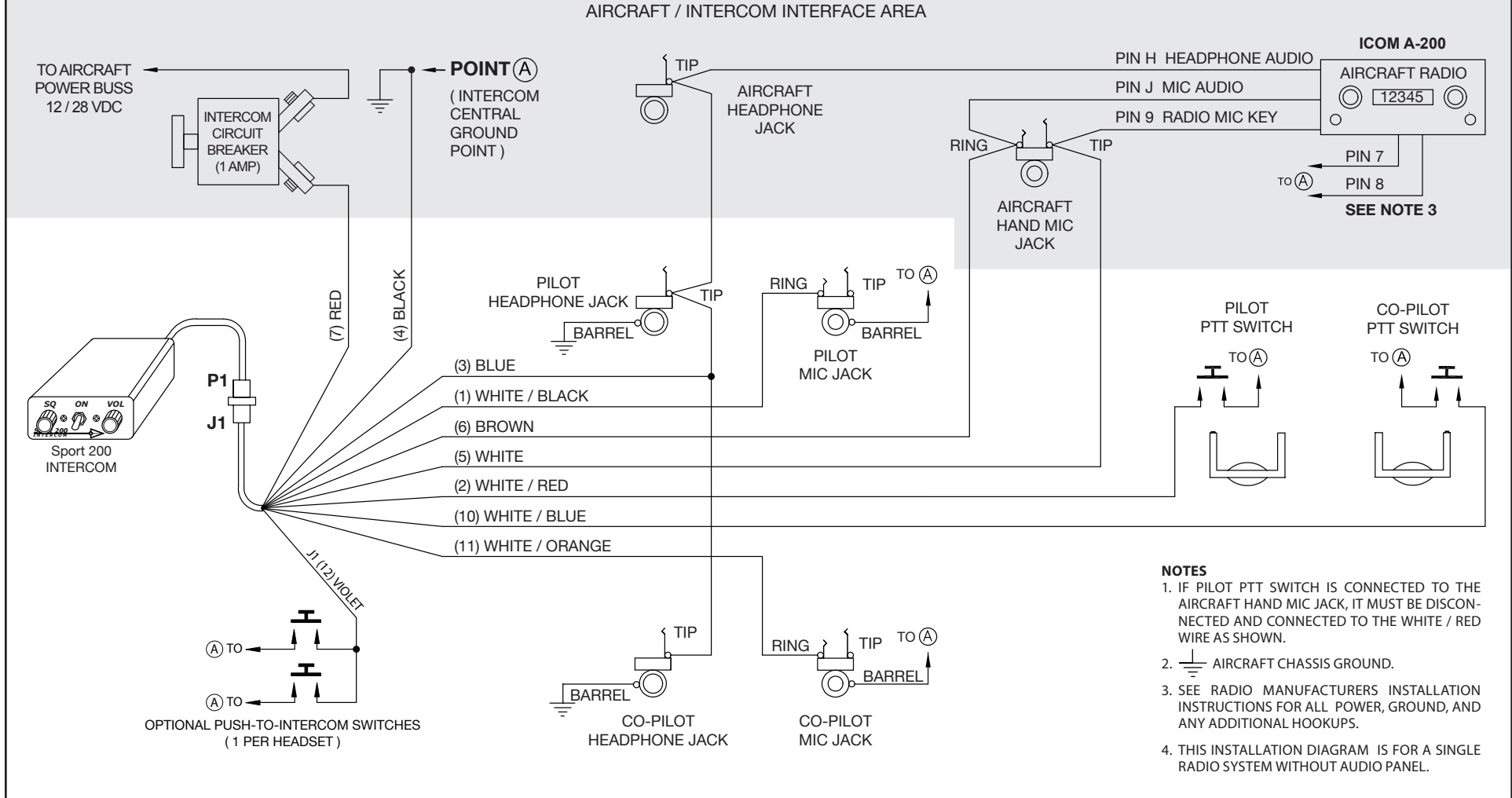
Sport 200 – ICOM A-200 Radio Installation Wiring Diagram
