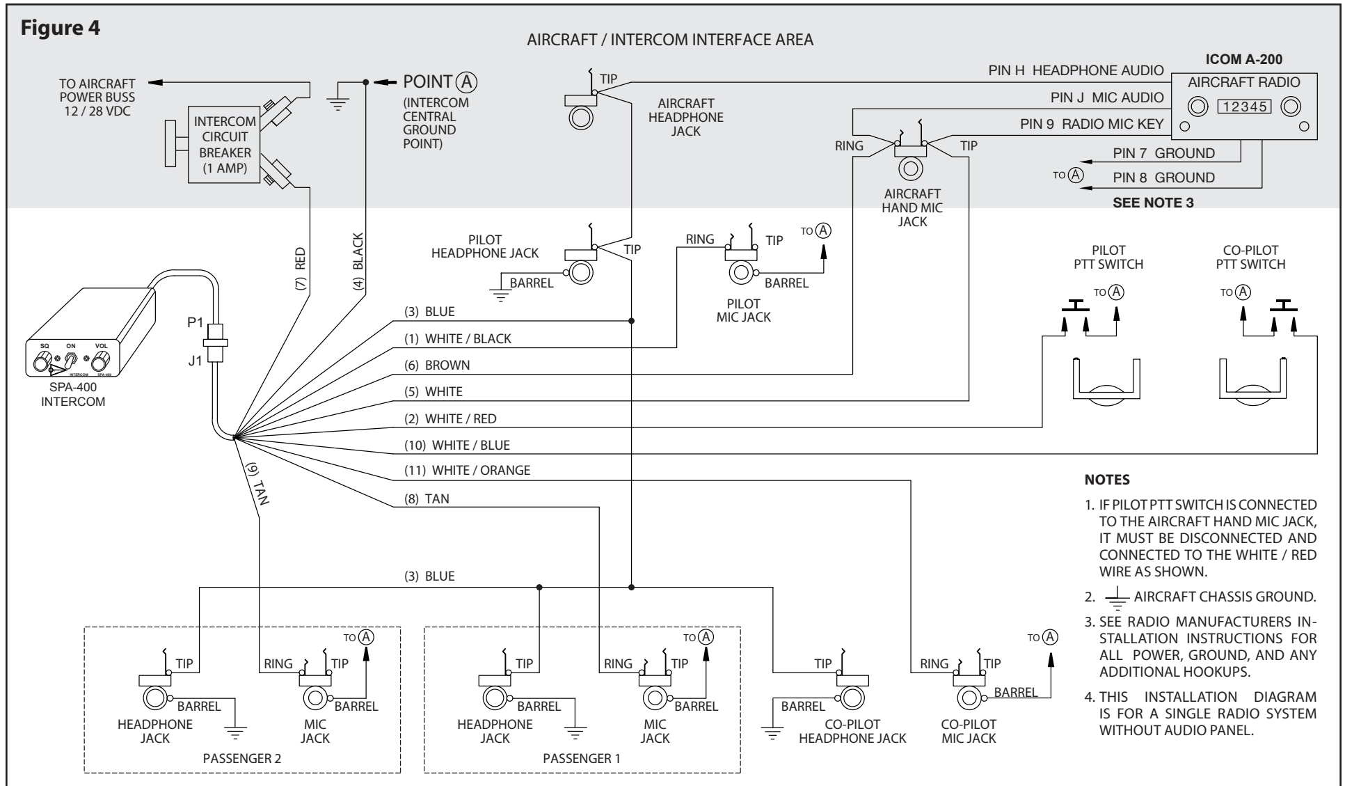
SPA-400 – ICOM A-200 Radio Installation Wiring Diagram
